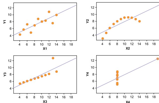
Figure 2 Correlation plot diagrams from Anscombe. 6 Copyright © 1973, American Statistical Association. All rights reserved. Reprinted with permission from Anscombe FJ. Graphs in statistical analysis. Am Stat . 1973;27:17–21.
