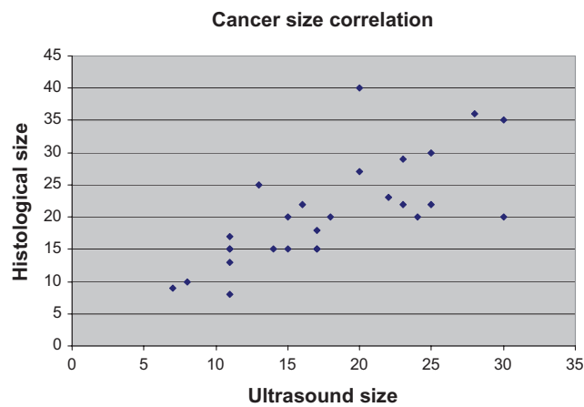
Figure 1 Plot of histological size compared to ultrasound measurement.
