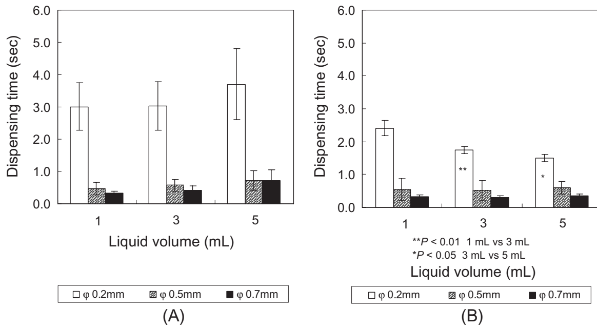
Figure 6 Dispensing time under condition of changing fluid volume, inner aperture diameter, and types of solution. Notes: Dispensing time (mean \pm SD) under a condition of fixed internal nozzle volume (30 mm 3 ) and pressure thrust load (0.05 MPa), and variable fluid volumes as well as inner aperture diameters. (□: 0.2 mm, ▨: 0.5 mm, ■: 0.7 mm) (A: filtrate water, B: surfactant solution); error bars indicate standard deviation. Asterisks indicate statistically significant difference: * P < 0.05 ; fluid volume of 3 mL vs fluid volume of 5 mL, ** P < 0.01 ; fluid volume 1 mL vs fluid volume of 3 mL.
