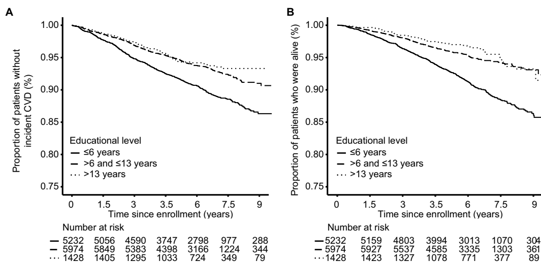
Figure 1 Kaplan-Meier curves for incident CVD (A) and all-cause mortality (B) by educational level.
