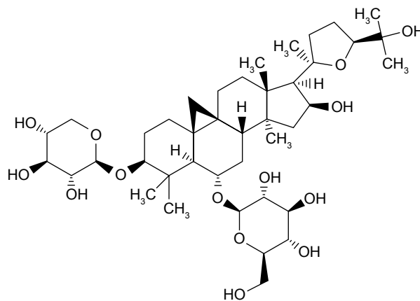
Figure 1 Chemical structure of AS-IV. Abbreviation: AS-IV, astragaloside IV.
