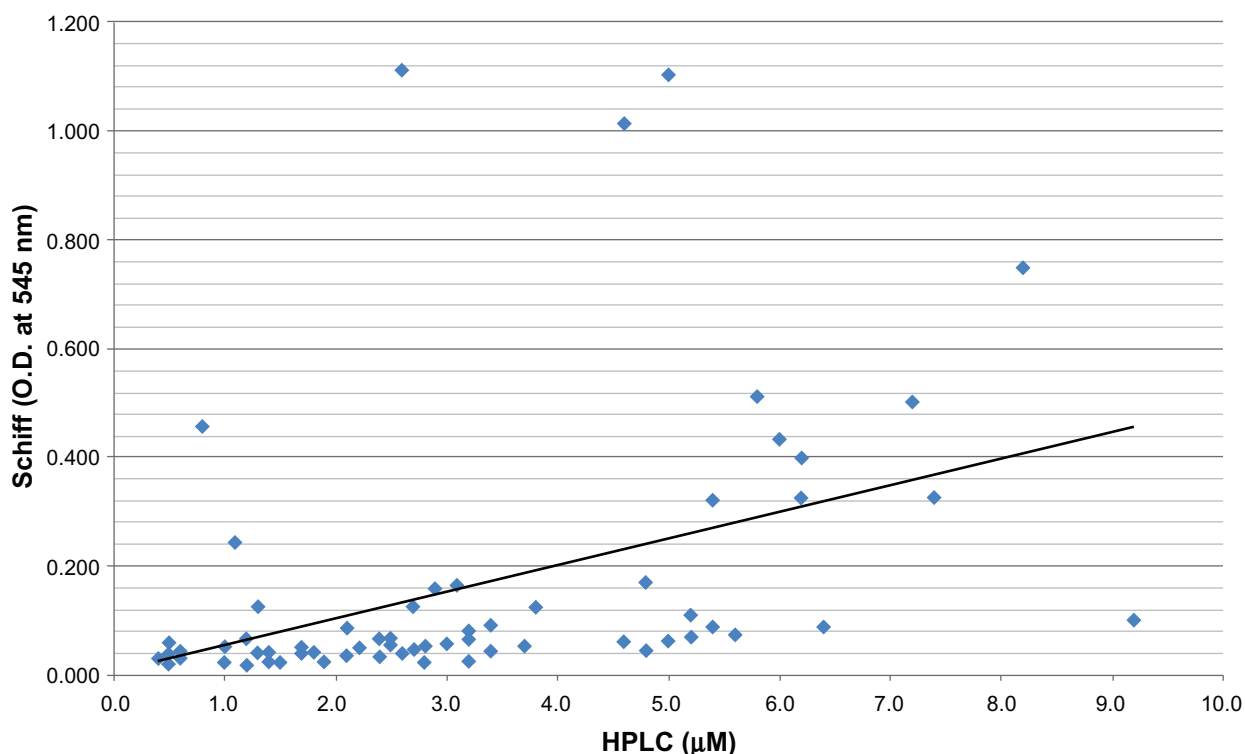
Figure 2 Comparison of the colorimetric Schiff assay results with the HPLC method.
