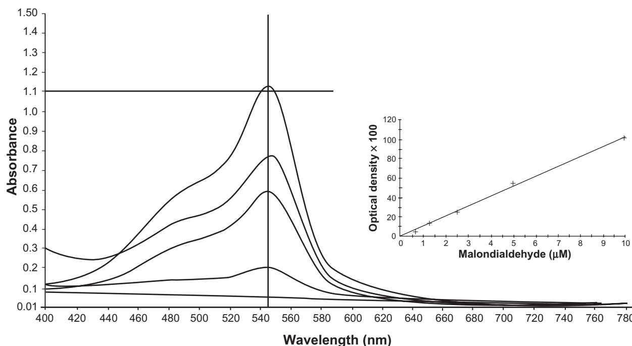
Figure 1 Absorption curve obtained by the Schiff method at different malondialdehyde concentrations.
