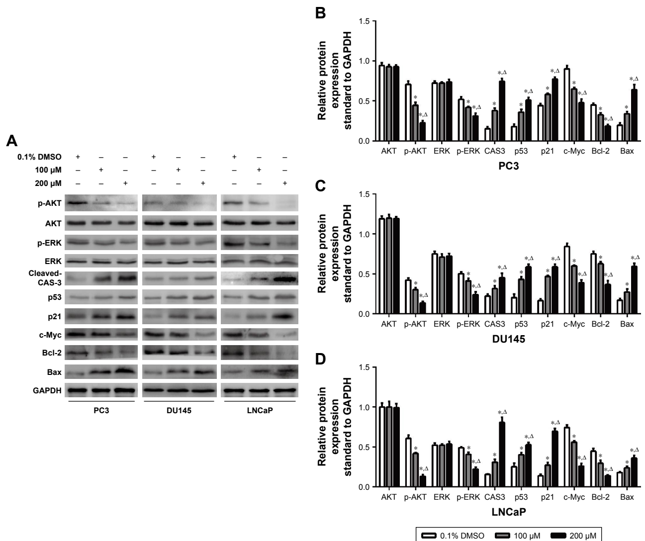
Figure 4 Western blot analysis. (A) Lysates from control and aloperine-treated PC3, DU145 and LNCaP cells were subjected to Western blot analysis using anti-p-AKT, AKT, p-ERK, ERK, c-Myc, cleaved caspase 3 (CAS3), Bcl-2, Bax and GAPDH. (B–D) Quantitative analysis of protein expression levels in prostate cancer cells treated with vehicle or aloperine (* P < 0.05 vs vehicle, \Delta P < 0.05 vs 100 \mu M, n = 3 ).
