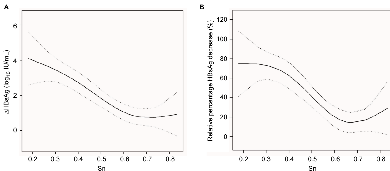
Figure 1 The non-linear negative relationship between baseline SHBs diversity ( S_n ) and \Delta HBsAg (A), relative percentage of HBsAg decrease (B).
