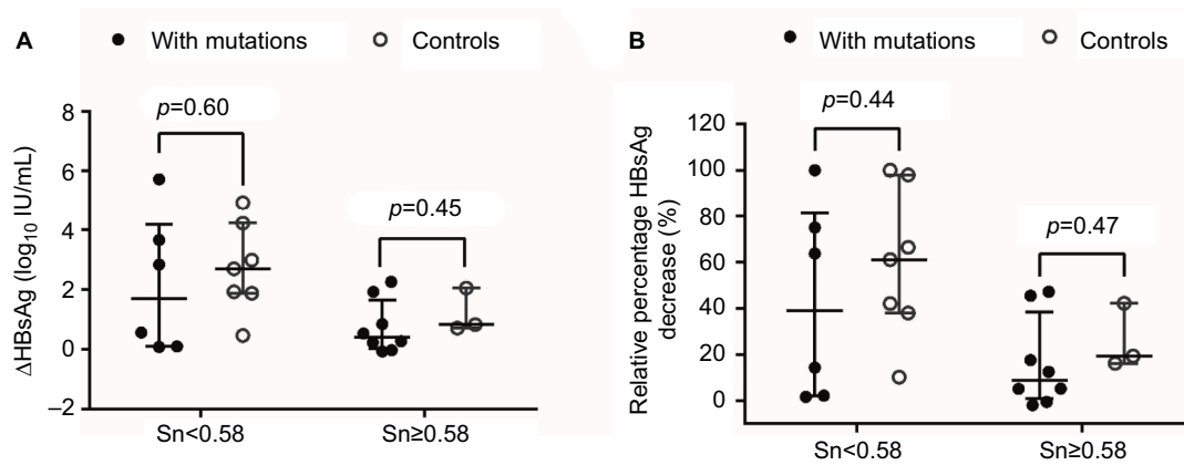
Figure 5 Effect of HBs-specific mutations on the \Delta HBsAg (A) and the relative percentage of HBsAg decrease (B) both in the Sn <0.58 and \geq 0.58 groups. Abbreviations: HBs, hepatitis B surface; HBsAg, hepatitis B surface antigen; Sn, normalized Shannon entropy.
