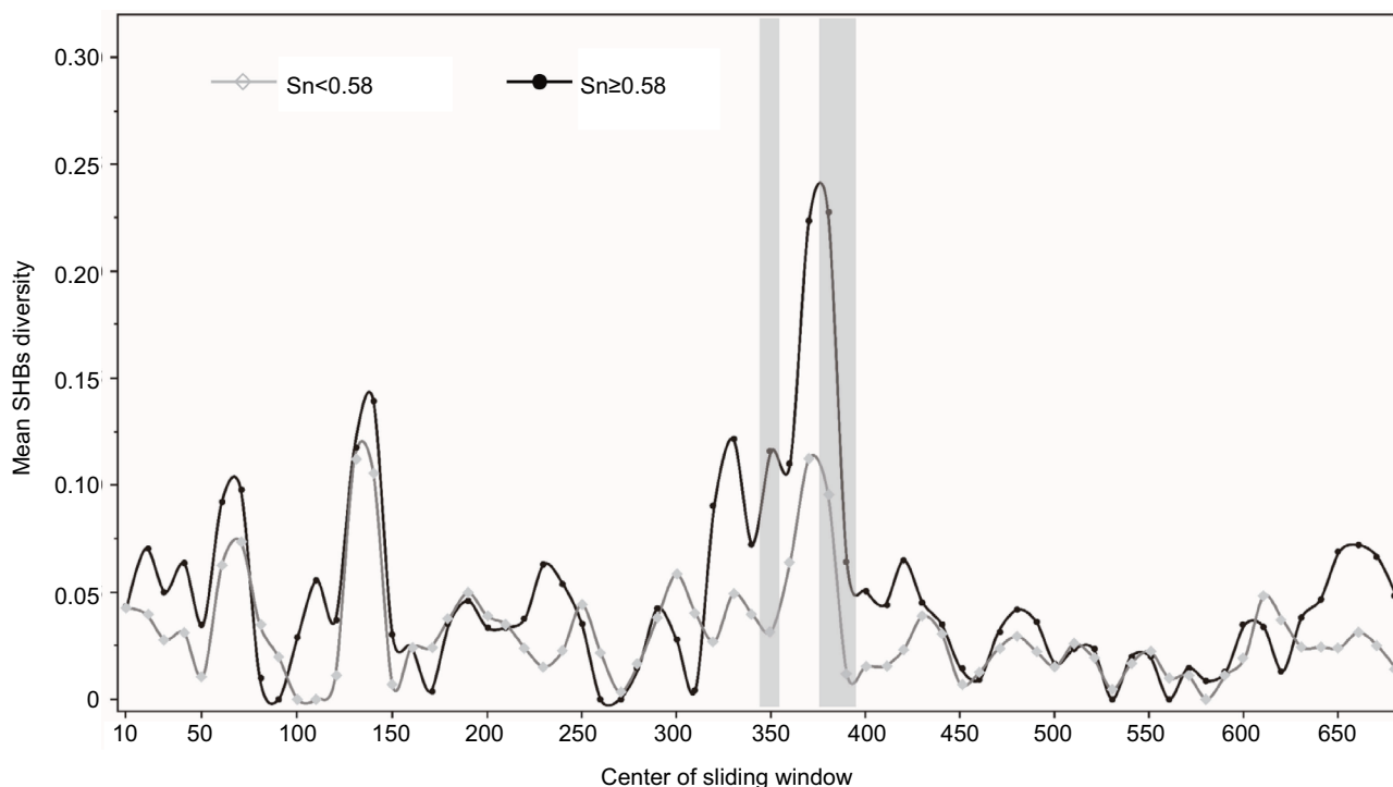
Figure 3 A sliding window analysis with overlapping 19-nucleotide segments migrating every 10 nucleotides for the small HBs gene. Notes: The gray line represents the S_n < 0.58 group, and the black line represents the S_n \geq 0.58 group. Grayed out segments correspond to statistically significant differences. Abbreviations: HBs, hepatitis B surface; SHBs, small hepatitis B surface protein; S_n , normalized Shannon entropy.
