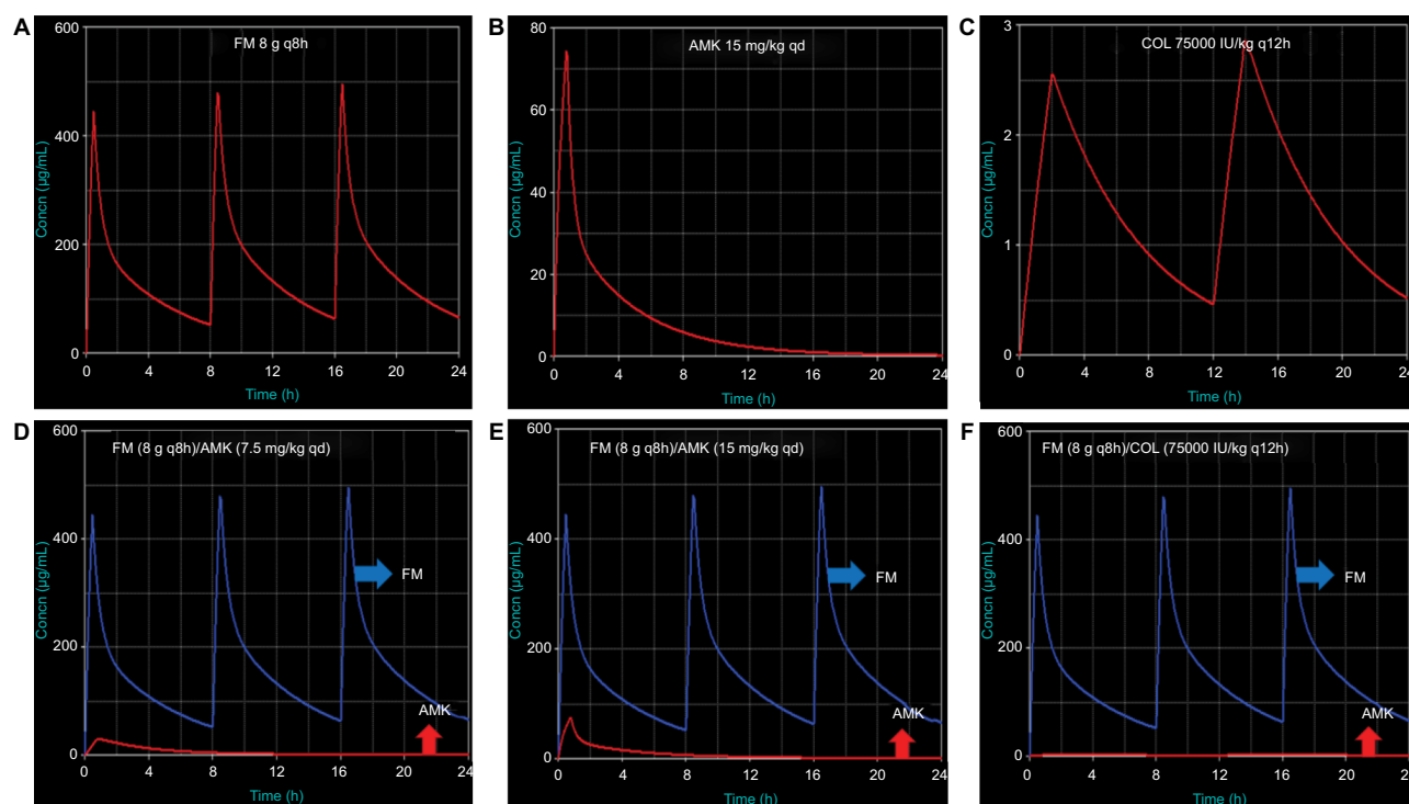
Figure S1 (A-F) The time–concentration curves of antibiotics in the Pharmacokinetics Auto Simulation System 400.
