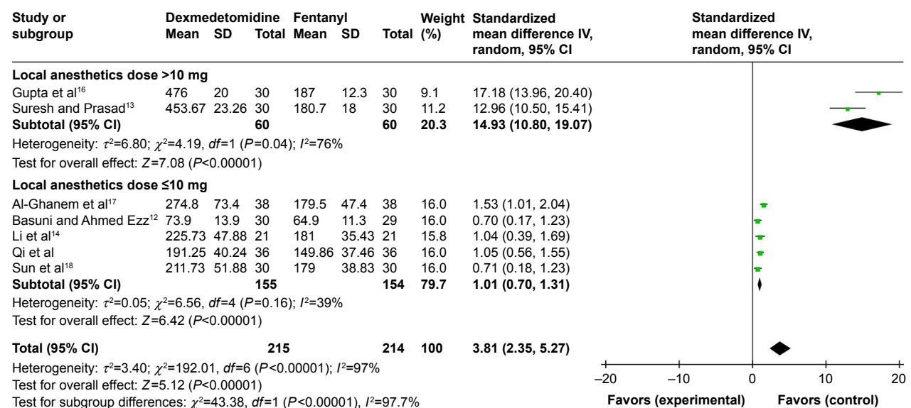
Figure 7 Forest plot for the subgroup analysis of duration of sensory block in minutes. Abbreviations: SD, standard deviation; CI, confidence interval; IV, inverse variance.
