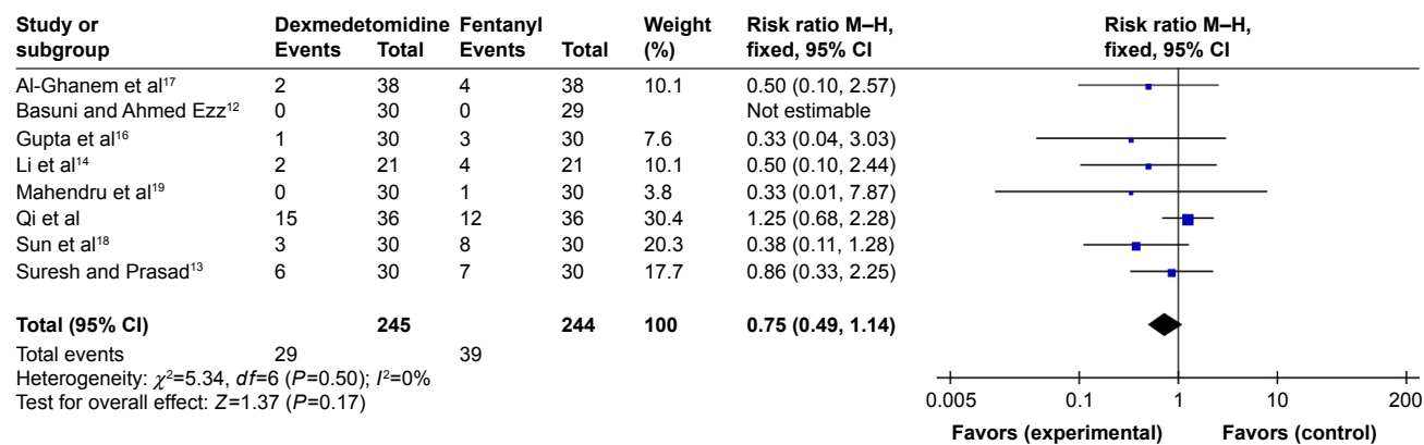
Figure 12 Forest plot comparing the incidence of side effects. Abbreviations: CI, confidence interval; M-H, Mantel-Haenszel.
