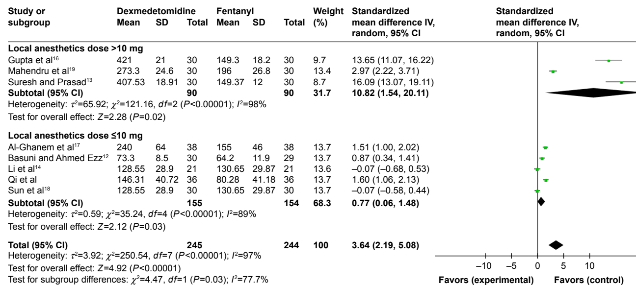
Figure 8 Forest plot for the subgroup analysis of duration of motor block in minutes. Abbreviations: SD, standard deviation; CI, confidence interval; IV, inverse variance.
