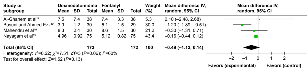
Figure 3 Forest plot for the onset of sensory block in minutes. Abbreviations: SD, standard deviation; CI, confidence interval; IV, inverse variance.
