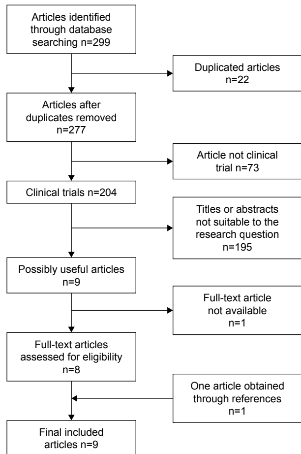
Figure 1 Flow chart for article selection in the meta-analysis.
