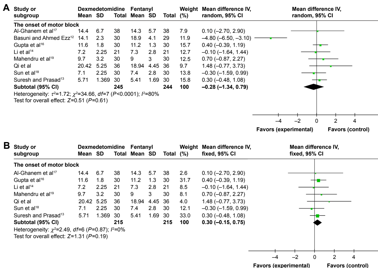
Figure 4 Forest plot for the onset of motor block in minutes (A), forest plot for sensitivity analysis of the onset of motor block in minutes (B).
