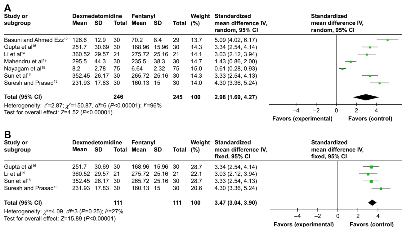
Figure 9 Forest plot for pain free period in minutes (A), forest plot for the sensitivity analysis of pain free period in minutes (B). Abbreviations: SD, standard deviation; CI, confidence interval; IV, inverse variance.
