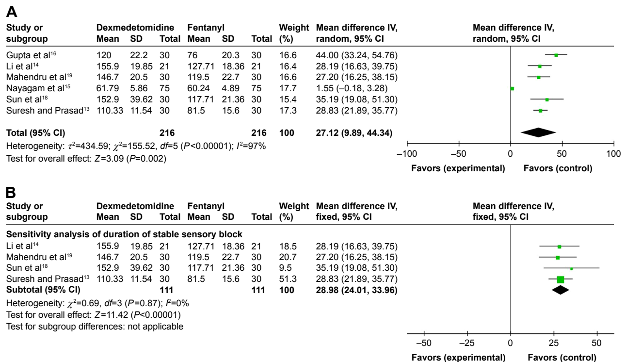
Figure 6 Forest plot for duration of stable sensory block in minutes (A), forest plot for the sensitivity analysis of duration of stable sensory block in minutes (B). Abbreviations: SD, standard deviation; CI, confidence interval; IV, inverse variance.
