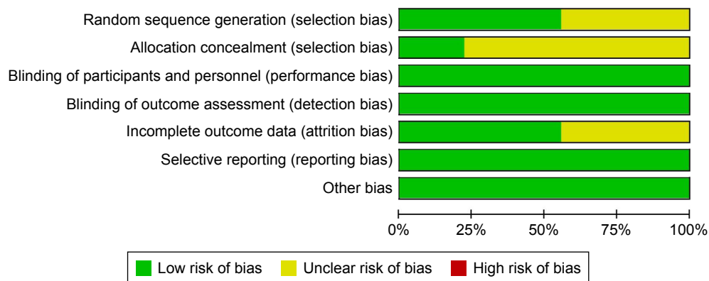
Figure 2 The risk of bias assessment of the included studies. Note: There were no high risk of bias found in these studies.
