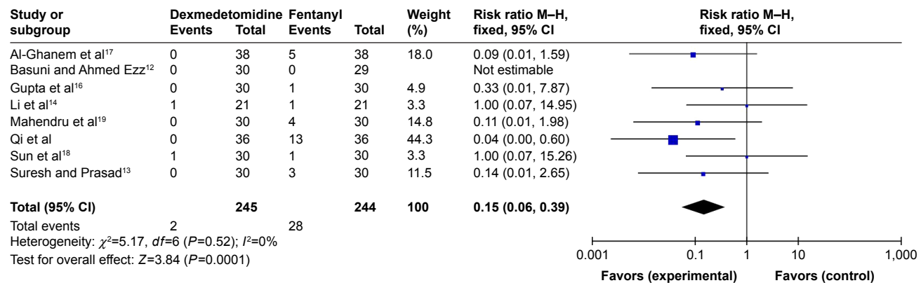
Figure 11 Forest plot comparing the incidence of pruritus. Abbreviations: CI, confidence interval; M-H, Mantel-Haenszel.
