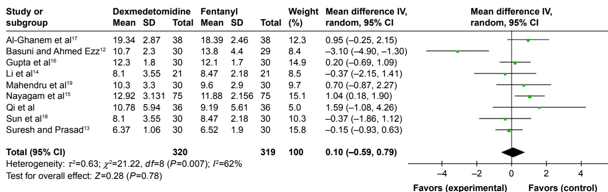
Figure 5 Forest plot for the time to peak sensory level.
