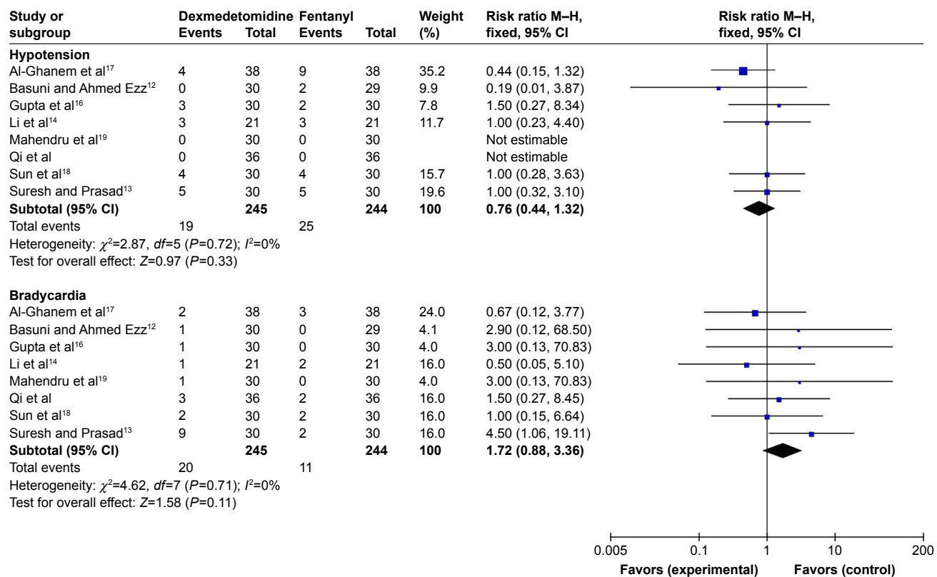
Figure 10 Forest plot comparing the incidence of hypotension and bradycardia. Abbreviations: CI, confidence interval; M-H, Mantel-Haenszel.
