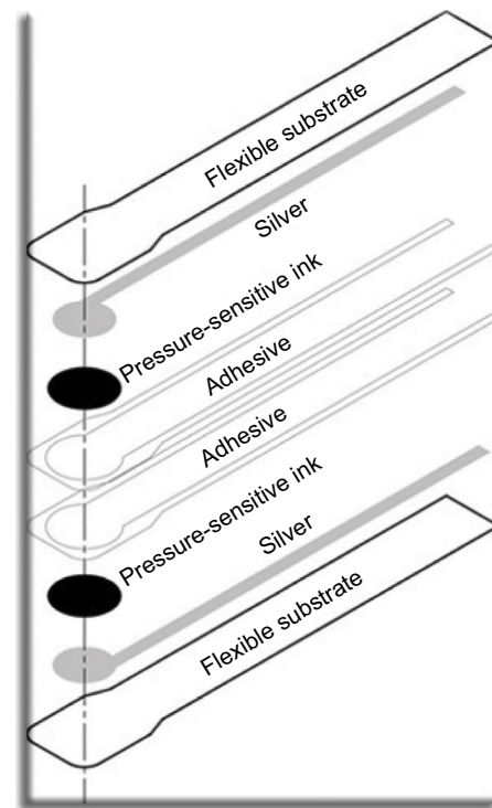
Figure 5 Schematic of sensor construction. Notes: Image courtesy of Tekscan, Inc.
