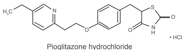
Figure 1 Pioglitazone chemical structure.
