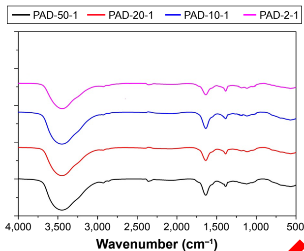
Figure S1 IR spectra of PAD-50-1, PAD-20-1, PAD-10-1, and PAD-2-1, recorded in the form of a KBr tablet (sample mass ratio 1:100). Note: PAD-X-Y, p(AAPBA- b -DEGMA) with DEGMA:pAAPBA molar ratios of X:Y. Abbreviations: DEGMA, diethylene glycol methyl ether methacrylate; IR, infrared; p(AAPBA), poly(3-acrylamidophenylboronic acid).
