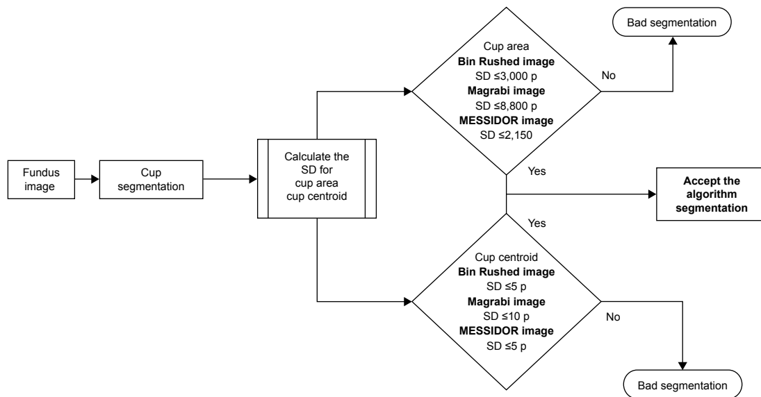
Figure 4 Flowchart for analysis of cup segmentation. Abbreviation: SD, standard deviation.
