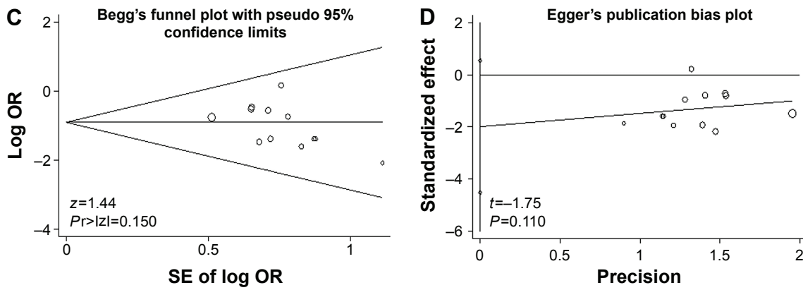
Figure S3 Publication bias.
