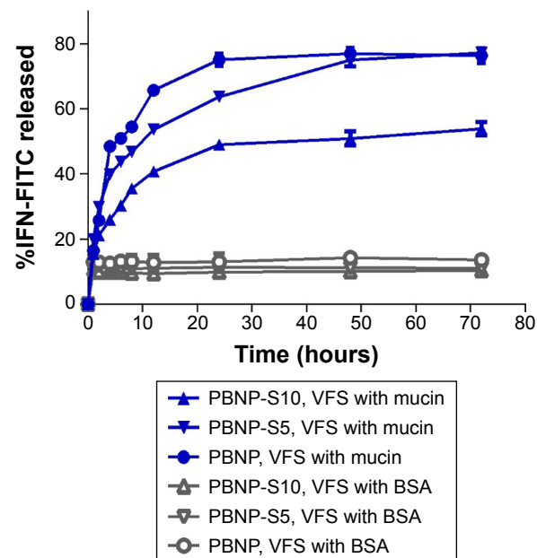
Figure S2 Drug loading and release of sulfated PBNPs with IFN-FITC as the model protein therapeutics.
