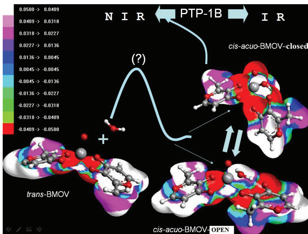
Figure 7 Energy diagram of the computed cis-trans conversion mechanism for the bioactive BMOV in its "closed-type cis-aquo"-form. In aqueous solution, the administered compound, trans-BMOV, intermediately converts into the "open-type cis-aquo-BMOV" complex being in equilibrium with the "closed-type cis-aquo-BMOV". Note, the activated transition complex of the reaction trans-BMOV + H 2 O remains hitherto unknown. NIR, normal insulin response; IR, state of insulin resistance.
