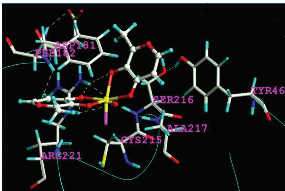
Figure 3 Result of the computed binding mode of the “closed-type cis-aquo-BMOV” complex at the active site (stick representation of 3D-model). Element color code: white C, light blue H, red O, dark blue N, yellow S or V, magenta LP.
