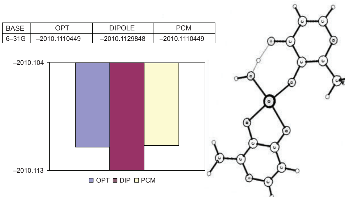
Figure 6 Results of the full optimization for the “open-type cis-aquo-BMOV” complex: (Top left) Total energies (in Hartree) for the basis set 6-31G. (Plot below) Total energy bar graphics (in Hartree): blue: without solvent; red: interaction model with a dipolar solvent; yellow: interaction model with a PCM-type solvent. (Right side) Schematic plot of the optimized structure.
