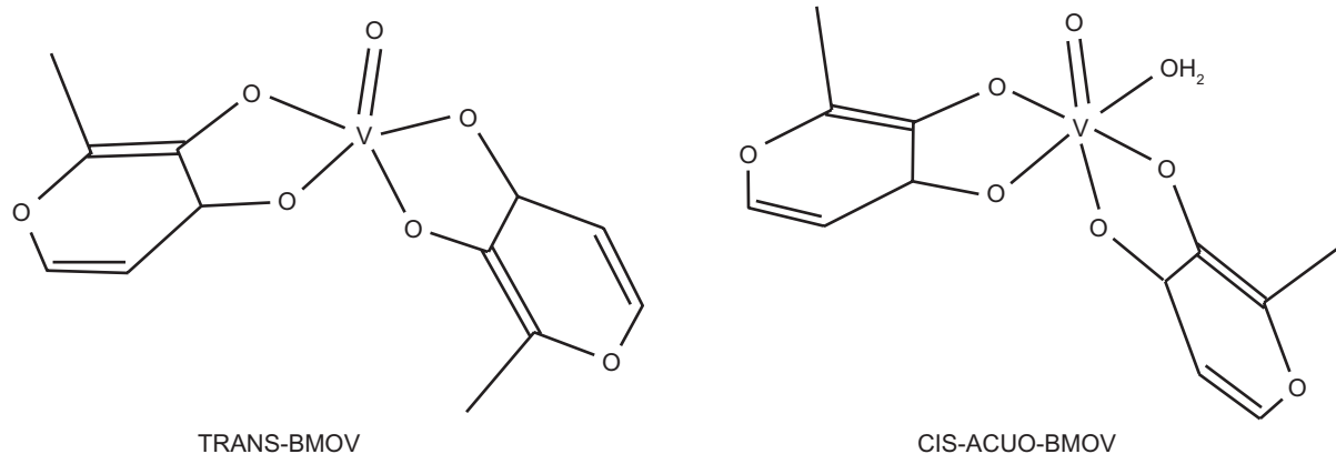
Figure 1 Structural representation of both isomers of BMOV in solution: (left) trans-BMOV, (right) the cis-acuo species where a solvent water moiety is attached to the central metal atom in the place of the electron lone pair. Despite the formal change in coordination geometries (trigonal bipyramidal to octahedral) due to the change of ligand number from 5 to 6 the over-all structure remains unchanged.
