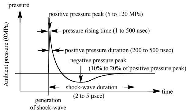
Figure 1 Pressure-time curve of a shock wave.
