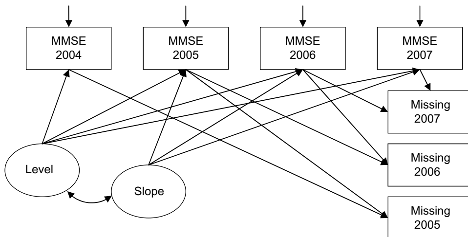
Figure 2 Latent growth curve model for Mini-Mental State Examination (MMSE) score under non-ignorable missing data assumption (Model 3).
