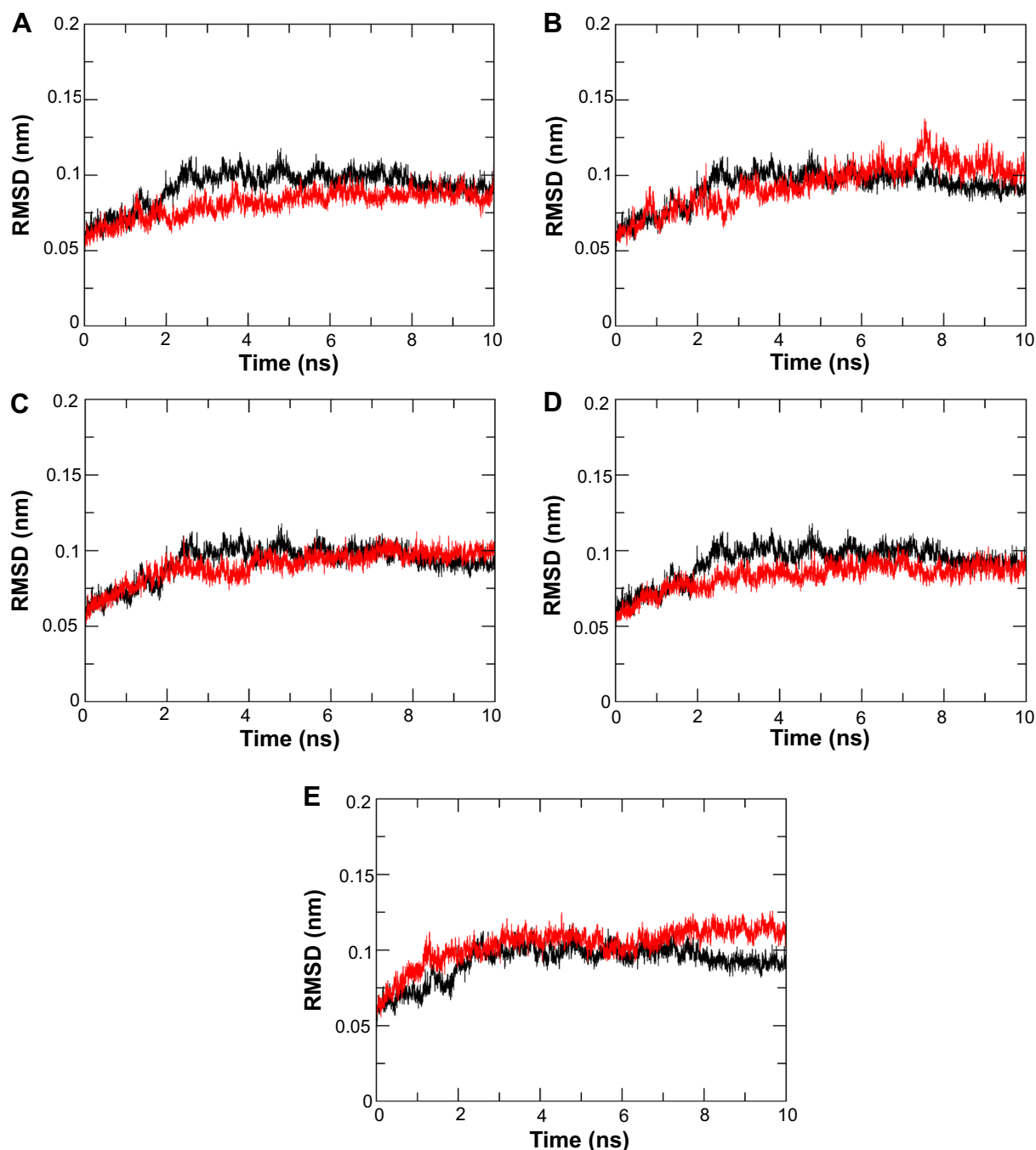
Figure 4 Root-mean-square deviation (RMSD) of backbone atoms of N9_R294K–inhibitor complexes. RMSD of oseltamivir carboxylate is shown in black. Notes: L-Arginine (A), aspartame (B), D-arginine (C), zanamivir (D), and benserazide hydrochloride (E).
