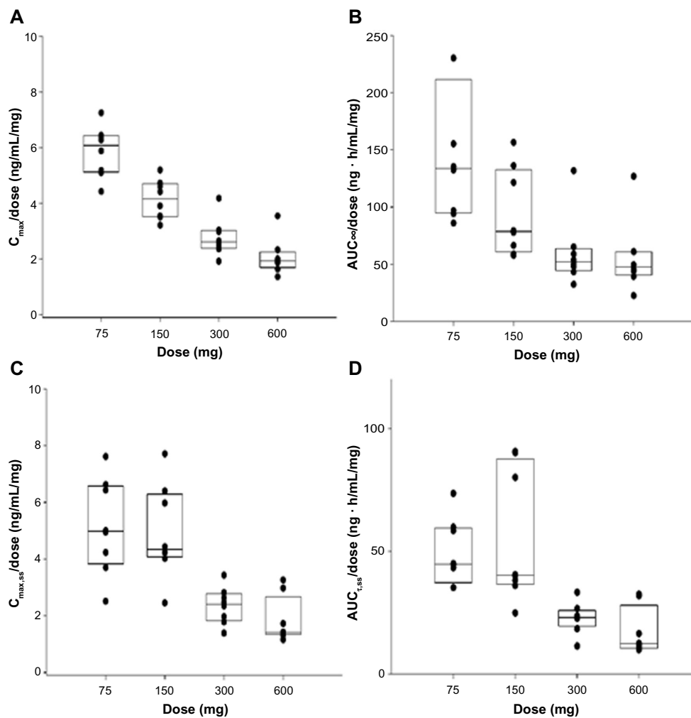
Figure 2 Comparisons of C_{max} /dose (A), AUC_{0-\infty} /dose (B), C_{max,ss} /dose (C), and AUC_{\tau,ss} /dose (D) with respect to KM-023 doses. (A and B) single dose; (C and D) multiple doses.
