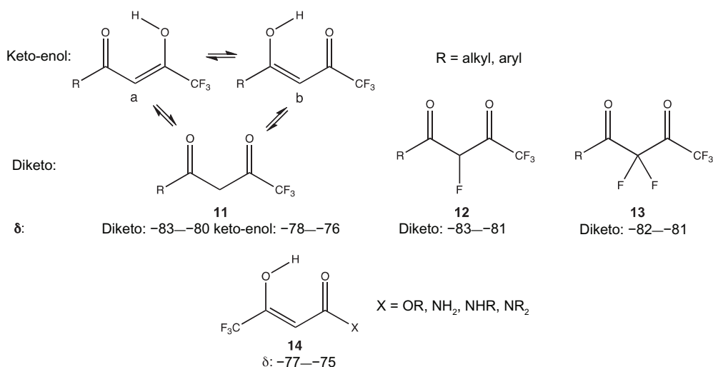
Figure 8 Acyclic trifluoromethyl- \beta -dicarbonyls.
