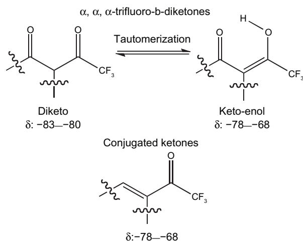
Figure 2 Shielding effects of substrate topology. Abbreviation: CF 3 , trifluoromethyl.
