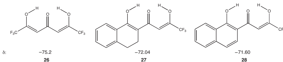
Figure 11 \alpha,\alpha -Trifluoromethyl-1,3,5-triketones. Abbreviation: \text{CF}_3 , trifluoromethyl.
