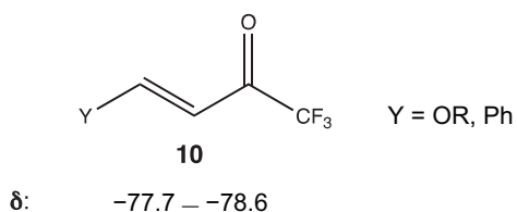
Figure 7 \alpha,\beta -Unsaturated trifluoromethyl ketones. Abbreviations: CF 3 , trifluoromethyl; OR, alkoxy; Ph, phenyl.
