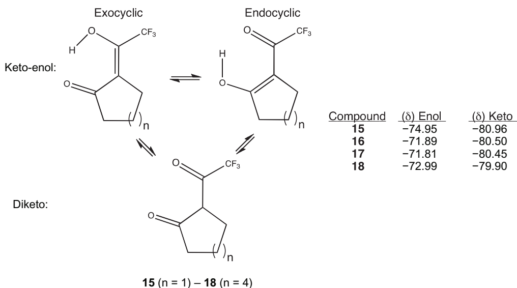
Figure 9 Trifluoroacetyl-cycloalkanones.
