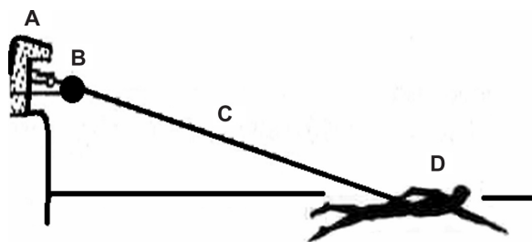
Figure 1 Schematic representation of the system used to determine the propulsive force of swimmer's arms.
