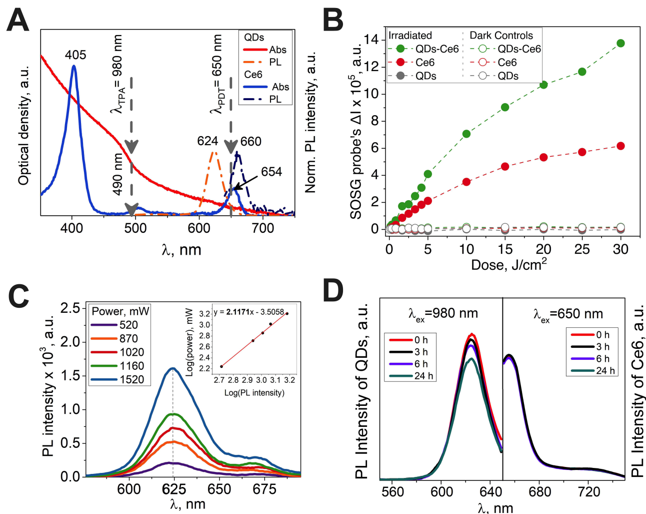
Figure 3 Characterization of the QDs-Ce6 nanocomplex. Normalized absorption and photoluminescence (PL) spectra of QDs and Ce6 solutions in RPMI-1640 medium (without phenol red) (A). The arrow at 490 nm indicates a wavelength used for SPA and corresponding TPA at 980 nm excitation of the samples. The line at 650 nm indicates the absorption band of Ce6 used for PDT therapy. (B) – Singlet oxygen generation capacity of QDs-Ce6 detected by SOSG probe. Samples were irradiated with xenon light (650/70 nm bandpass filter). (C) – Photoluminescence of QDs-Ce6 nanocomplex in RPMI-1640 medium after excitation by 980 nm laser with varying power (from 520 mW to 1520 mW). Insert of (C) shows derived data and mathematical approximation (straight line function) for assessment of multiphoton process. The stability of the nanocomplex was assessed by measuring PL spectra after different time intervals of incubation: 0, 3, 6, and 24 hours in RPMI-1640 medium (D). Two excitation wavelengths were used: \lambda_{ex} = 980 nm and \lambda_{ex} = 650 nm.
