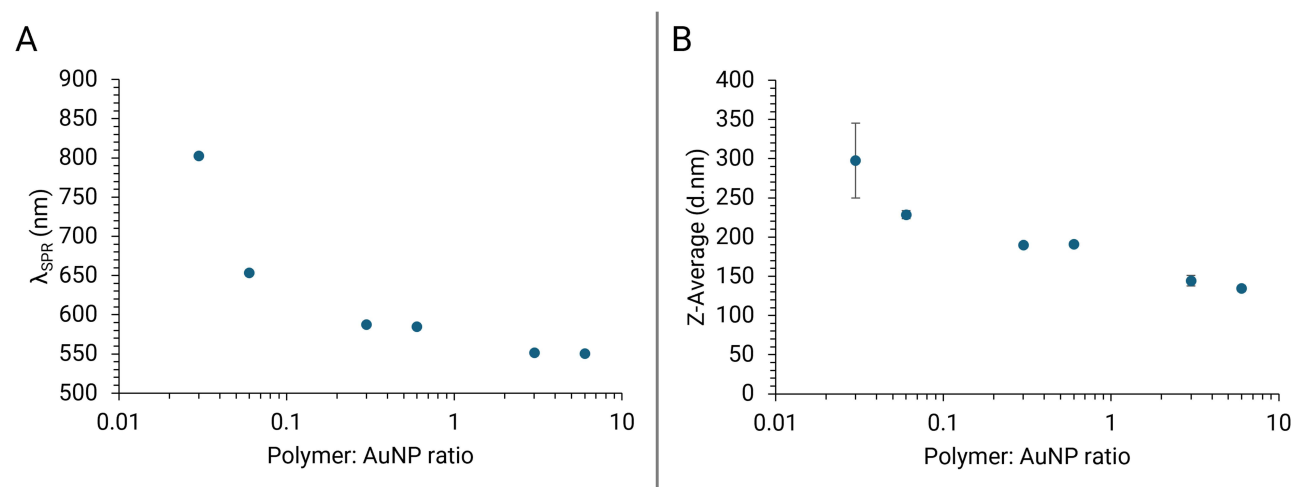
Figure 5 Effect of varying polymer: AuNP ratio on physicochemical properties of AuNC. Position of Surface Plasmon Resonance (SPR) peak (A), and Z-average hydrodynamic diameter (B).
