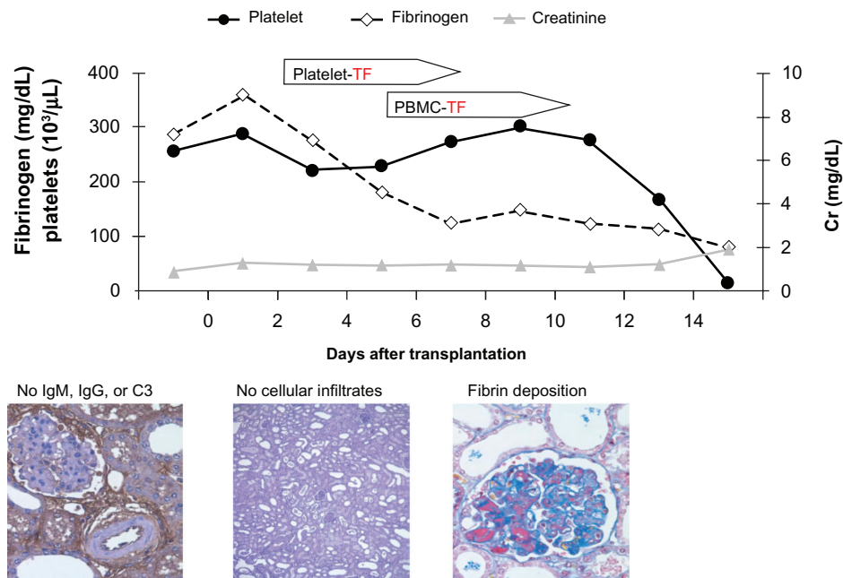
Figure 4 Correlation between platelet count and fibrinogen level (indicating the development of a consumptive coagulopathy) and tissue factor expression on platelets and peripheral blood mononuclear cells (PBMC) in a baboon following GTKO/CD46 pig-to-baboon kidney transplantation.
