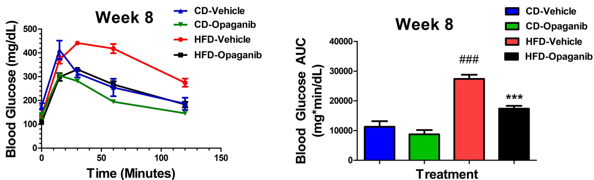
Figure 3 Effect of opaganib on HFD-induced glucose intolerance. Left Panel: Male C57BL/6 mice were given a CD and treated with either Vehicle (▲, n = 3) or 100 mg/kg Opaganib (▼, n = 3) or a HFD and treated with either Vehicle (●, n = 8) or 100 mg/kg Opaganib (■, n = 9) once daily, 5 days/week. Blood glucose levels were measured and values indicate the mean ± SEM at the indicated time of sampling. HFD-Opaganib was significantly reduced (p < 0.05 for time = 15 min and p < 0.001 for all other time points) compared with HFD-Vehicle. Right Panel: Mean ± SEM values for the blood glucose concentration AUCs are shown. ### p < 0.001 vs CD-Vehicle and *** p < 0.001 vs HFD-Vehicle.
