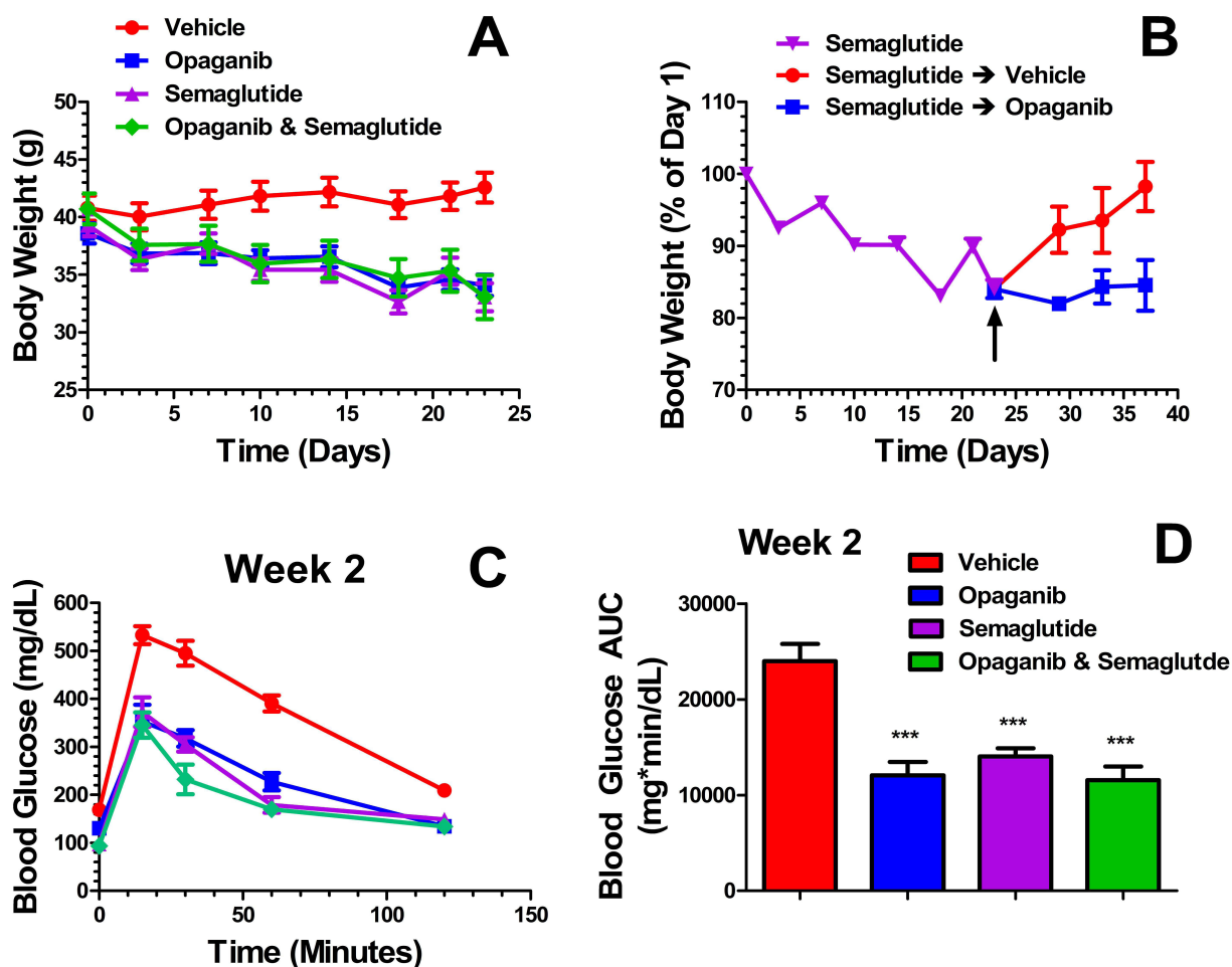
Figure 9 Effects of opaganib and semaglutide on body weight and glucose tolerance in obese mice. (A) Male C57BL/6J mice were given HFD for 18 weeks and the treated with either Vehicle (●, n = 8), opaganib (■, n = 6), semaglutide (▲, n = 6) or opaganib plus semaglutide (◆, n = 7). Mice were weighed on the indicated days and the mean \pm SEM values are shown. (B) Semaglutide-treated mice were randomized on Day 23 (Arrow) to Vehicle (●) or opaganib (■) and weights were measured until Day 27. (C) Glucose tolerance curves at 2 weeks of treatment are shown. Mean \pm SEM values are shown. (D) Values for the blood glucose concentration AUCs at 2 weeks are shown. *** p < 0.001 vs Vehicle.
