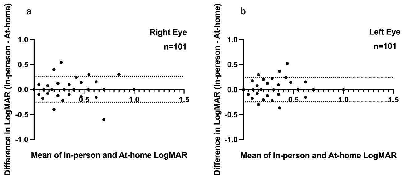
Figure 2 (a) The Bland-Altman Plot of the Right Eye. Bland-Altman plot of the right eye demonstrating the mean in-person and at-home logMAR value on the x axis and difference between in-person and at-home logMAR value on the y axis. The dotted line represents the 95% confidence interval calculated by \pm 1.96 standard deviations of mean. Sample size included all 101 study participants ( n = sample size). (b) The Bland-Altman Plot of the Left Eye. Bland-Altman plot of the left eye demonstrating the mean in-person and at-home logMAR value on the x axis and difference between in-person and at-home logMAR value on the y axis. The dotted line represents the 95% confidence interval calculated by \pm 1.96 standard deviations of mean. Sample size included all 101 study participants ( n = sample size).
