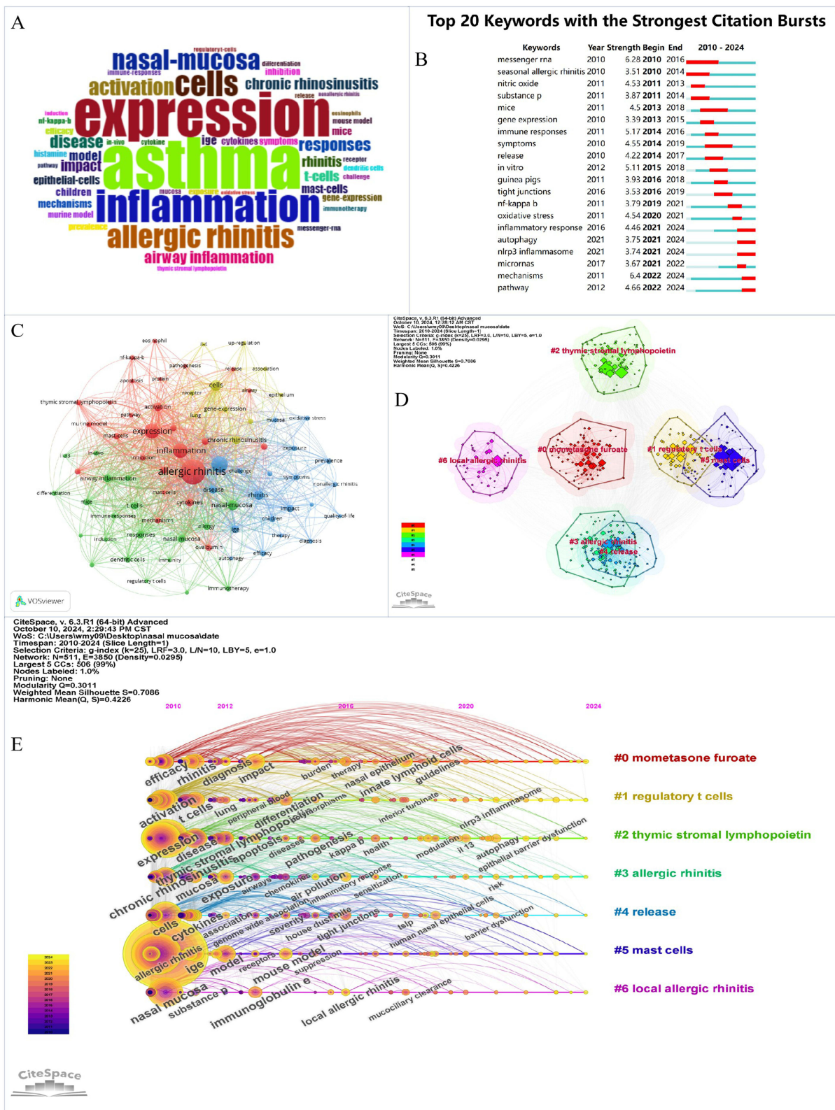
Figure 10 Keywords and burst analysis. (A) WordCloud; (B) Top 20 keywords with the strongest citation bursts; (C) Keywords co-occurrence network; (D) Keywords clustering map; (E) Timeline view of keywords.
