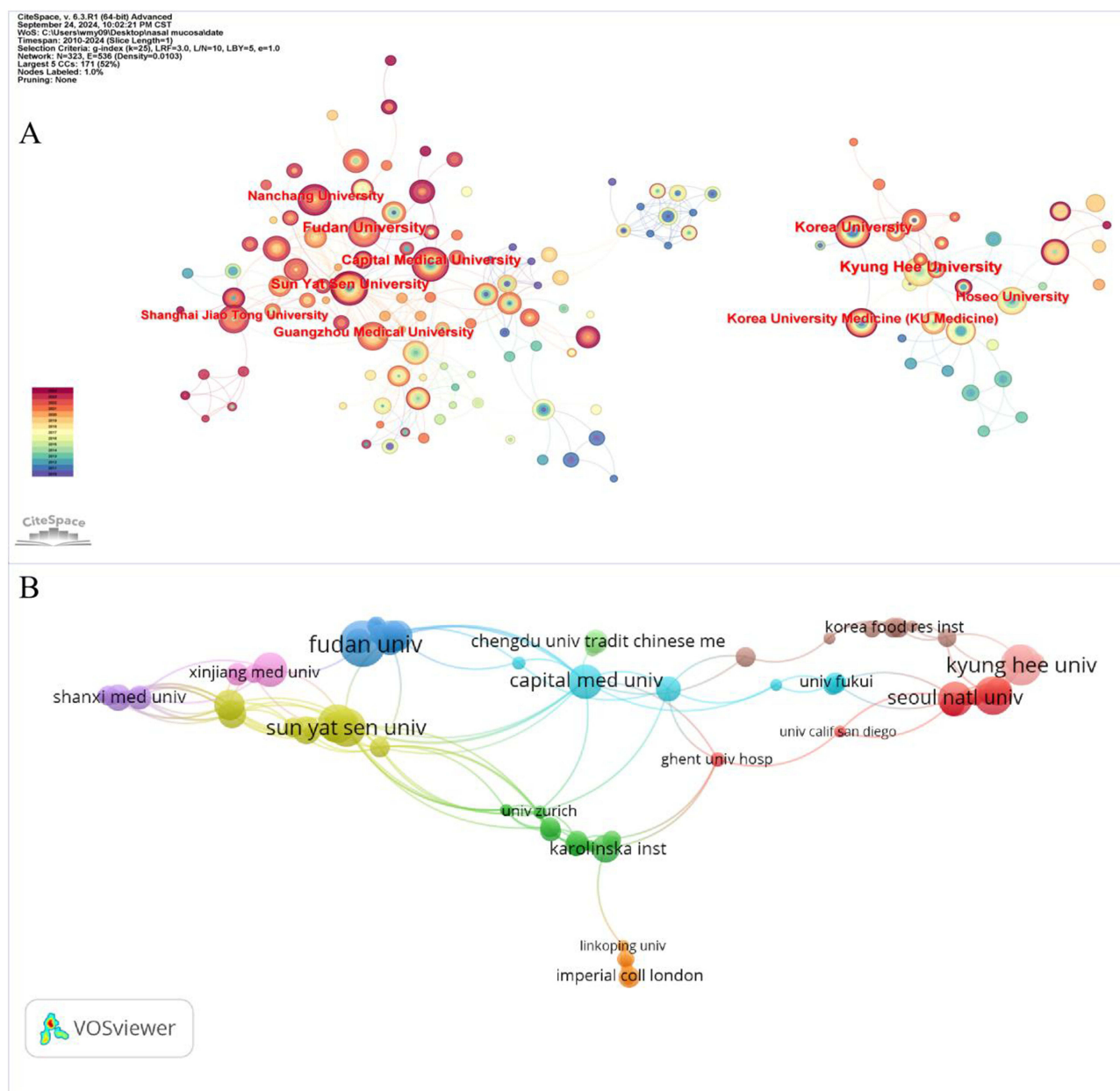
Figure 6 Institutions analysis. (A) Citespace's visualization map; (B) VOSviewer's visualization map.
