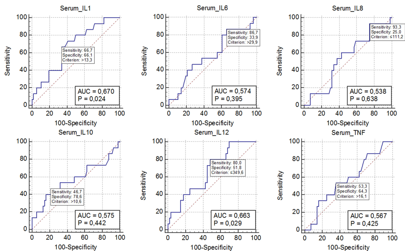
Figure 2 ROC curves showing serum levels of cytokines IL-1, IL-6, IL-8, IL-10, IL-12 and TNF- \alpha in relation to colposcopic lesion area (greater or less than 1cm 2 ).
