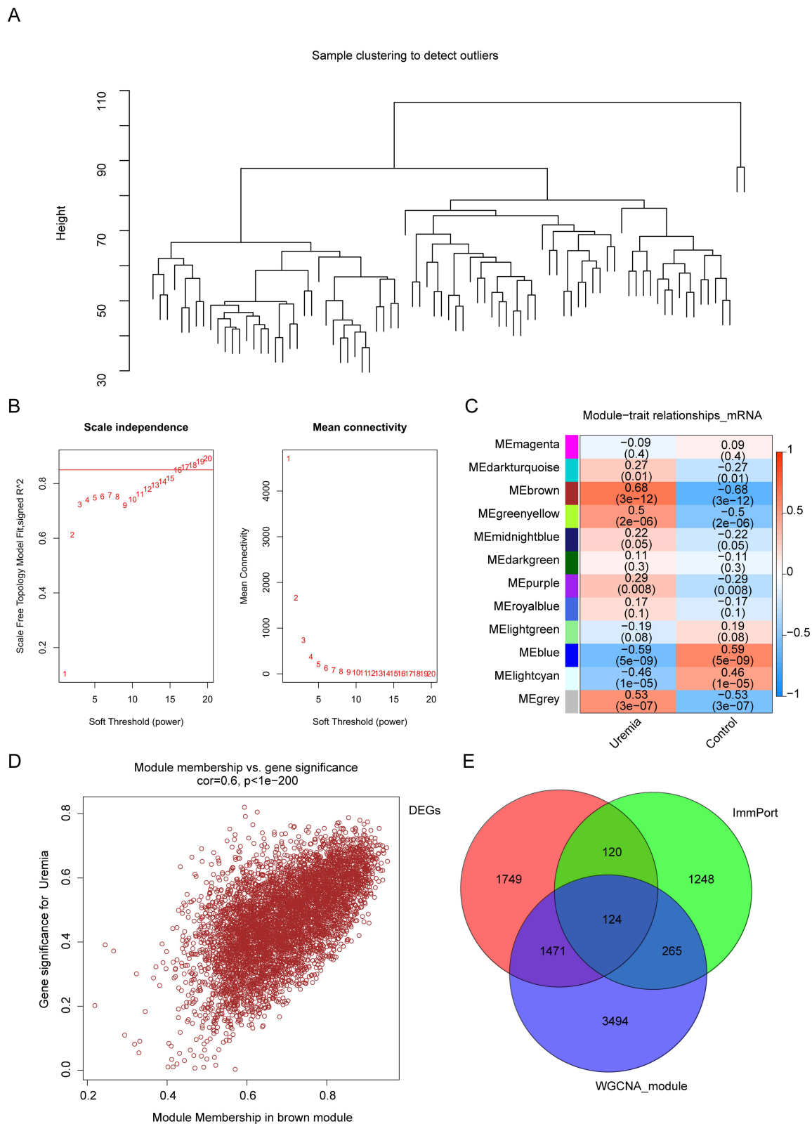
Figure 2 Weighted gene co-expression network analysis (WGCNA). (A) Sample cluster dendrogram of 20 control samples and 63 uremia samples based on their expression profile. (B) Analysis of mean connectivity of each \beta value from 1 to 20. \beta = 17 was chosen for subsequent analyses as it has the biggest mean connectivity when the scale-free fit index is up to 0.85. (C) Heatmap of the module-trait correlation. The brown module exhibited the highest correlation with uremia. (D) Scatter plot of correlation between genes and traits in the MEbrown module. (E) Venn diagram representation of the intersection of differentially expressed genes (DEGs), immune-related genes from the ImmPort database, and the brown module. In total, 124 core DEGs were identified.
