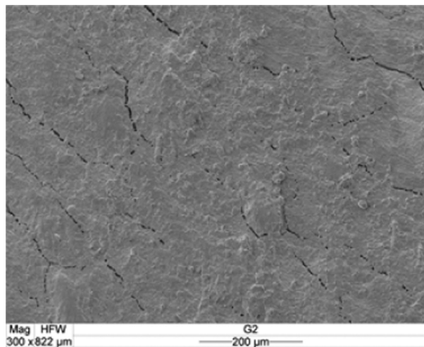
Figure 4 Half-tooth, untreated.
