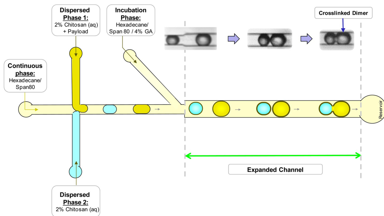
Figure 6 Schematic of the microfluidic device used to synthesize dimer like Janus particles. Reprinted with permission from Lu AX, Jiang K, DeVoe DL, et al. Microfluidic assembly of Janus-like dimer capsules. Langmuir . 2013;29(44):13624–13629. Copyright (2013) American Chemical Society. 80
