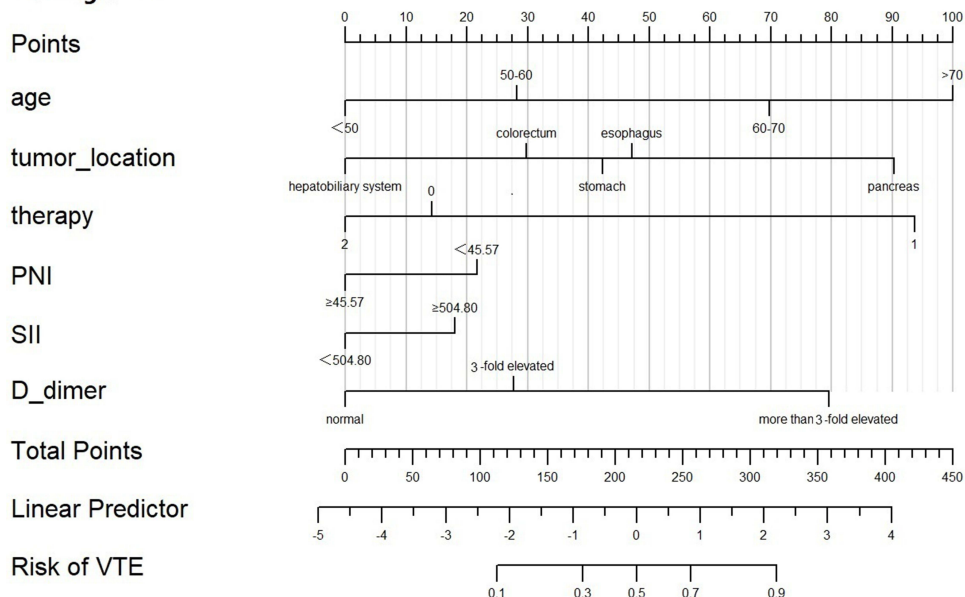
Figure 3 The nomogram of the model B.
