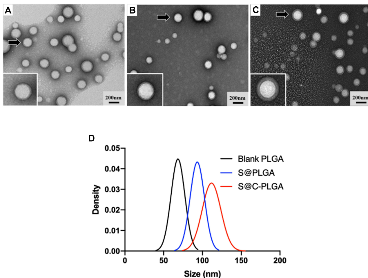
Figure 1 Evaluation of nanoparticles in term of size. Transmission electron micrographs of blank PLGA NPs (A), S@PLGA NPs (B) and S@C-PLGA NPs (C). Insets show a single particle denoted by arrow. (D) The normalized size distributions of nanoparticles obtained from the analysis of TEM images ( n=100 ) that were quantified using ImageJ software version 2.0.
