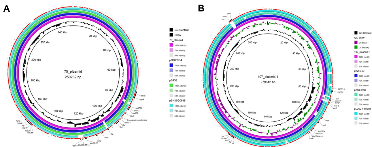
Figure 1 Circular representation of the studied plasmids. GC content and GC Skew were represented on the distance scale (in kbp) on the inner map. Each plasmid was compared to its most closely-related plasmid. The red arc around the map indicated ORFs. Certain important genes were also indicated on the ring. The hp is short for hypothetical protein. (A) 75_Plasmid alignment map; (B) 107_Plasmid-1 alignment map.
