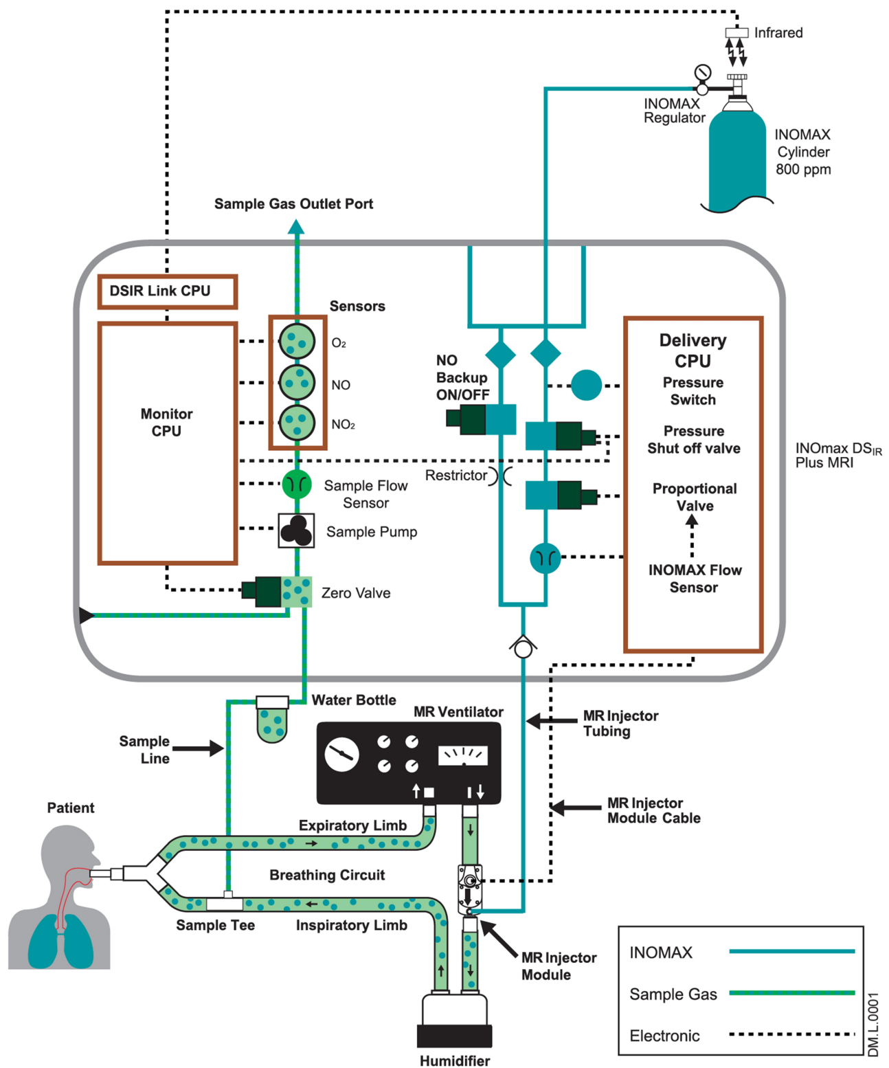
Figure 1 Schematic diagram of the INO max DSIR Plus Magnetic Resonance Imaging System. Reproduced with permission from INOmax DSIR ® Plus MRI Operation Manual, Mallinckrodt Pharmaceuticals, Hampton, NJ, USA; 2015. 24
