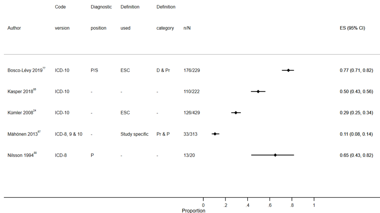
Figure 4 Sensitivity for heart failure diagnoses from studies which reported the number of records confirmed positive and the total number of records.
