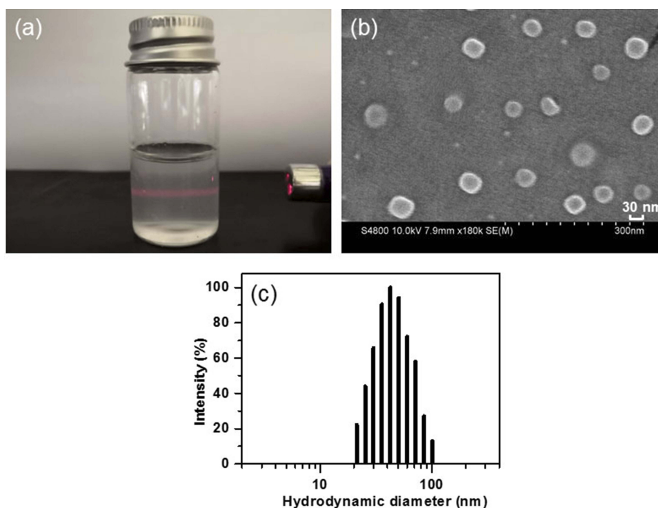
Figure 4 (A) Photo of the solution of CSAD-VB 12 /insulin nanoparticles, (B) SEM image of CSAD-VB 12 /insulin nanoparticles, (C) hydrodynamic diameter distribution of CSAD-VB 12 /insulin nanoparticles.
