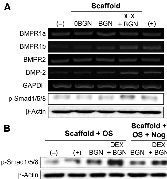
Figure 6 BMP-2 signaling pathway analyses.
